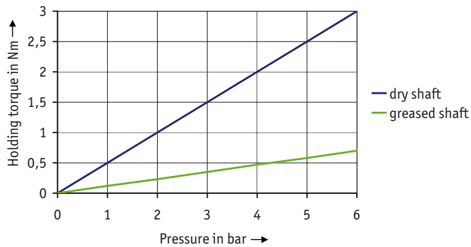
Achievable holding torques
